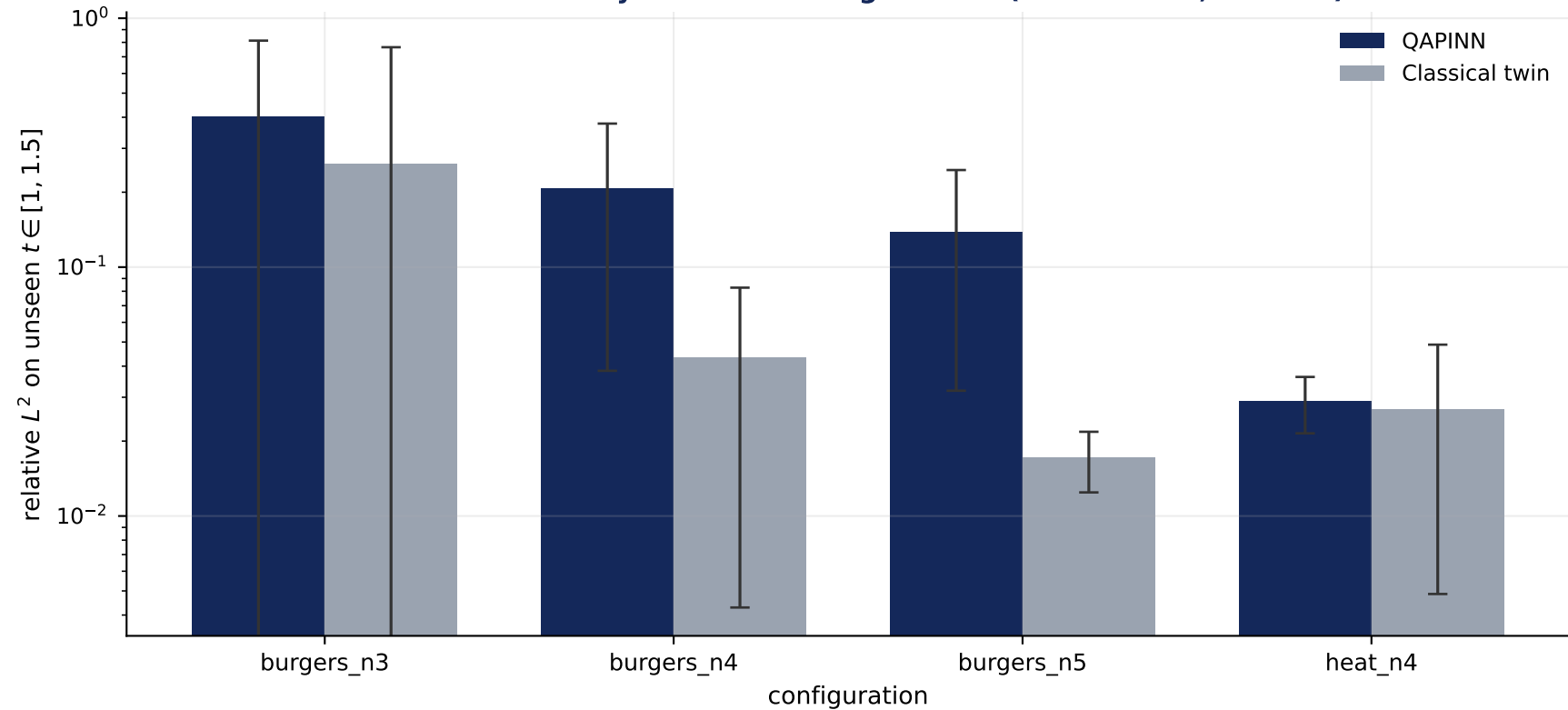
Generalization beyond the training domain (mean \pm s.d., 5 seeds)
